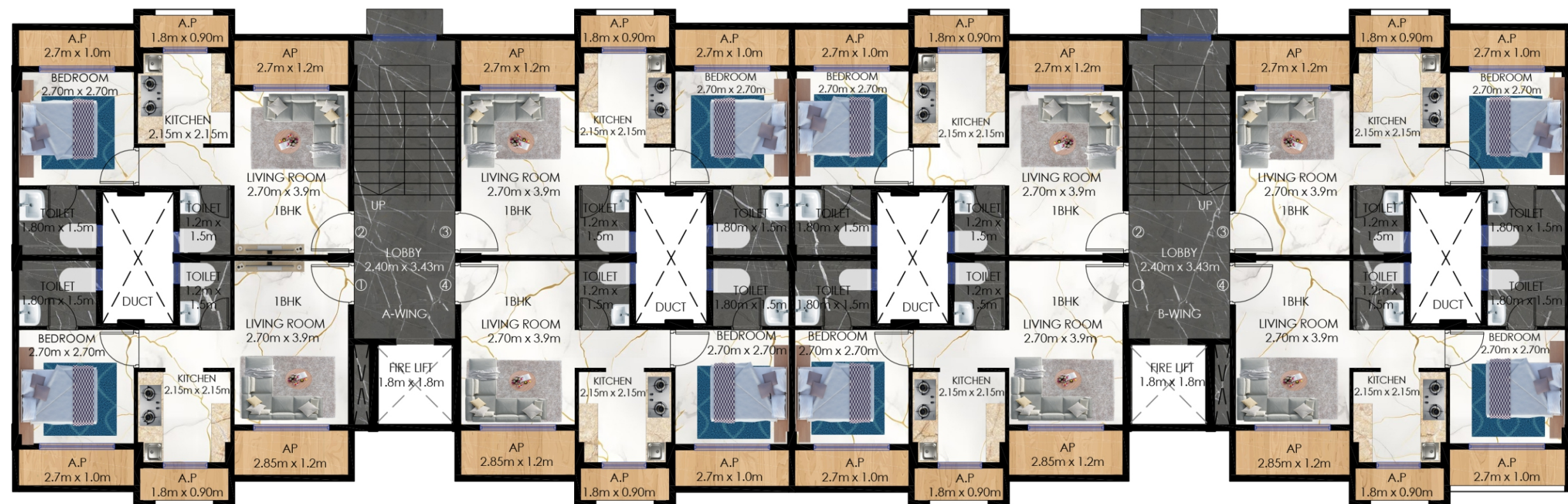
TYPICAL FLOOR PLAN BLDG No.1
